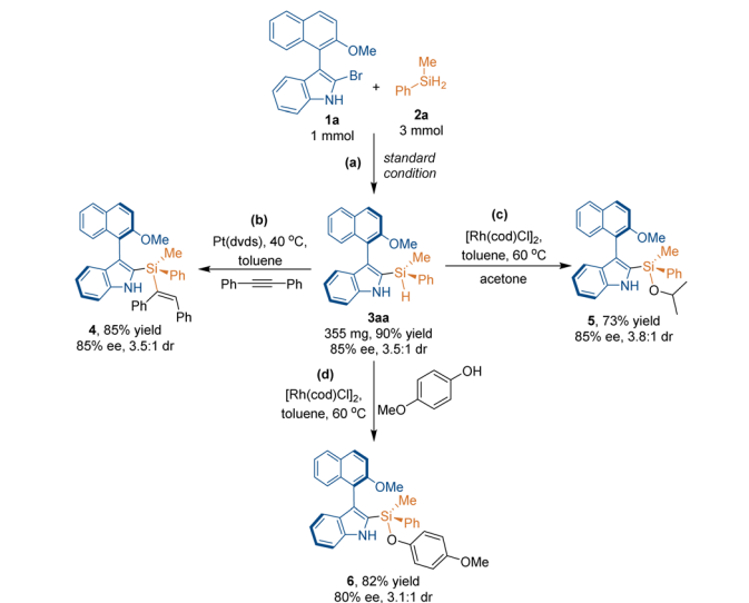
Scheme 1 One-mmol-scale reaction and downstream transformations.
