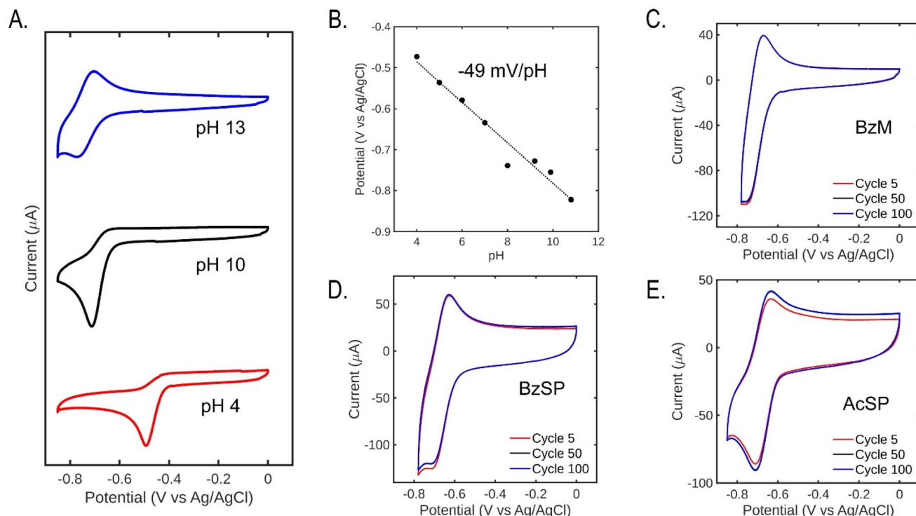
Fig. 2 Cyclic voltammetry of 5 mM pyridinium mediators at 100 \text{ mV s}^{-1} under argon. (A) Cyclic voltammograms of BzM in various buffers with 1 M KNO 3 . (B) Pourbaix diagram of BzM. (C–E) Long-term cyclic voltammograms in unbuffered 1 M KNO 3 of BzM, BzSP, and AcSP.
