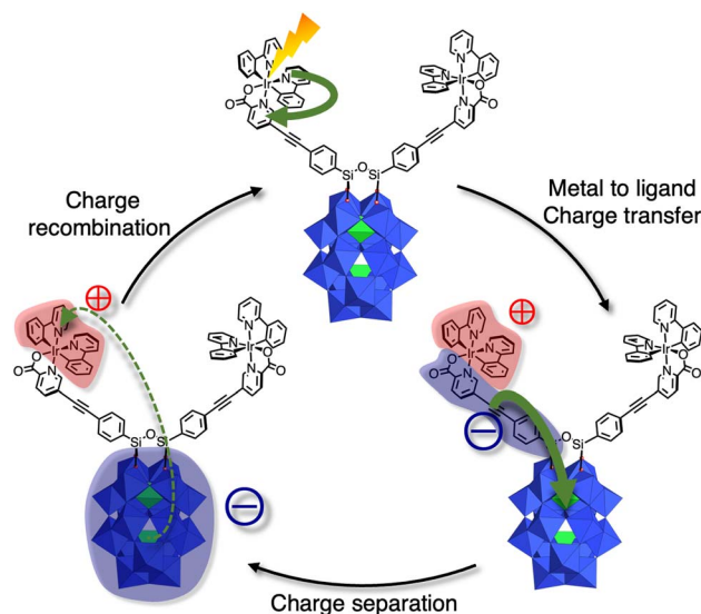
Fig. 5 Directionality in the photoinduced electron transfers of the POM-Ir(III) assembly [P_2W_{17}O_{61}(O(SiC_{36}H_{23}O_2N_3Ir_2))]^{6-} , conferred by the heteroleptic character of the Ir(III) complex. The red and blue cloud respectively represent the localization of the positive and negative charges in the different excited states. 51
