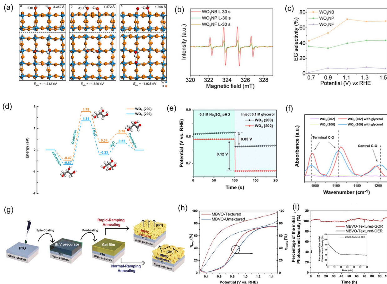
Fig. 14 (a) Representation of the atomic structures of the lowest-energy • OH adsorption on twinning W atoms of different facets, in which, from left to right, the sequence is facets of (010), (100), and (001). The corresponding adsorption energy is presented at the bottom. (b) EPR analyses of • OH in the presence of WO 3 NB, WO 3 NP or WO 3 NF after light illumination (c) PEC CH 4 -to-EG conversion selectivity at various potential using the photoanode of WO 3 NB, WO 3 NP or WO 3 NF. Reproduced with permission. 108 Copyright 2021, John Wiley and Sons. (d) Energy profiles derived from DFT calculation of glycerol oxidation on WO 3 at the facets of (200) and (202). (e) The comparison of WO 3 in OCP change between facets of (200) and (202) in a supporting electrolyte with subsequent injection of 0.1 M glycerol. (f) FT-IR absorbance spectra of the C–O bond vibration peaks of WO 3 photoanodes with predominant facets of (200) and (202) in a Na 2 SO 4 solution with or without glycerol. Reproduced with permission. 69 Copyright 2022, American Chemical Society. (g) Schematic representation of the process of synthesising textured and untextured MBVO. (h) The \eta_{\text{sep}} and \eta_{\text{int}} ( \eta_{\text{trans}} ) of textured and untextured MBVO. (i) The PEC stability of textured MBVO under glycerol oxidation and OER (inset) conditions. Reproduced with permission. 115 Copyright 2024, John Wiley and Sons.
