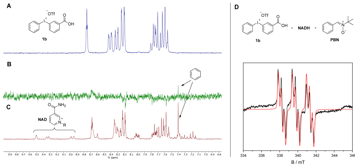
Fig. 4 (A) ^1\text{H} -NMR spectrum of 1b (methanol- d_4 / \text{D}_2\text{O} at 200 MHz). (B) ^1\text{H} -CIDNP spectrum recorded 30 min after mixing 1b and NADH. (C) ^1\text{H} -NMR recorded 30 min after the spectrum B. (D) CW-EPR during the reaction of 1b , NADH, and PBN overlaid with the simulated spectrum.
