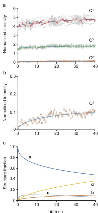
Fig. 6 Kinetic analysis for the a to b to c to d pathway of the reaction mechanism shown in Fig. 5. (a and b) Plots showing the fitting of the intensities of the ^{29}\text{Si} Q^4 , Q^3 and Q^2 signals calculated using the Avrami–Erofe'ev equation (blue lines) to the (normalised) experimental intensities (shown as circles with error bars) extracted from the in situ ^{29}\text{Si} NMR spectra recorded as a function of time in Fig. 2a. The estimated error bars are \pm 10\% of the experimental value. (c) Plot showing the relative amounts of a , b , c and d as a function of time.
