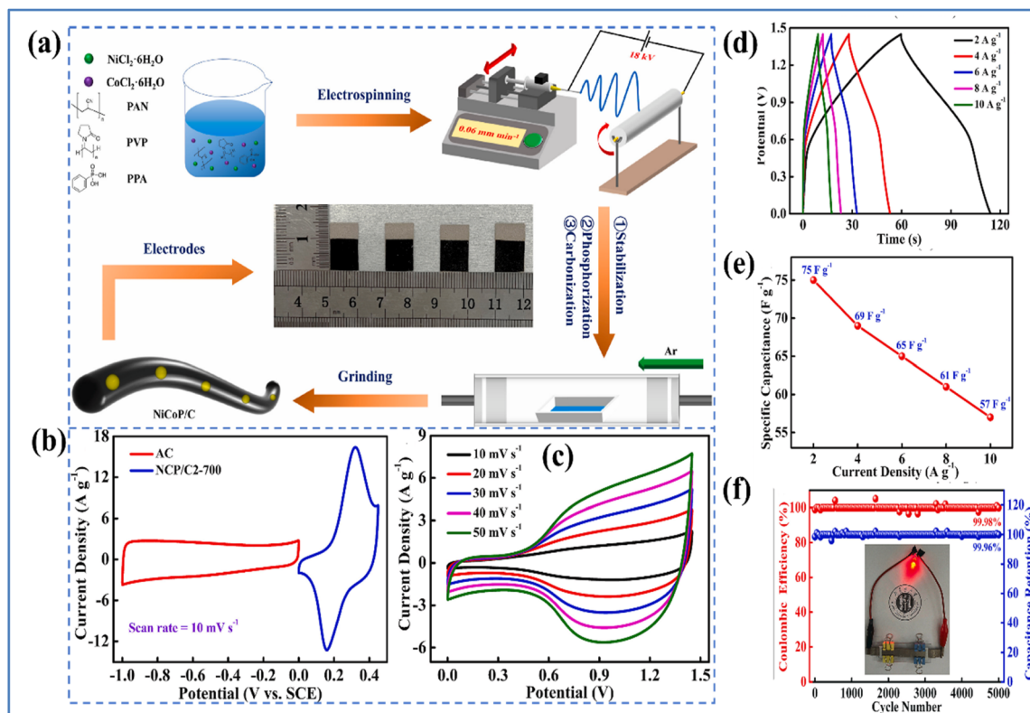
Fig. 6 (a) Schematic representation of the preparation of NiCoP/C composite (b) CV curves of NCP/C2-700 and AC at a \nu of 10 mV s -1 (c) CV curves at different \nu (d) GCD curves (e) rate capability curve of NCP/C2-700//AC device (f) cycling life and \eta of NCP/C2-700//AC at 10 A g -1 and a digital photo of a red LED illuminated by NCP/C2-700//AC device (reproduced from ref. 34 with permission from Elsevier© 2024).
