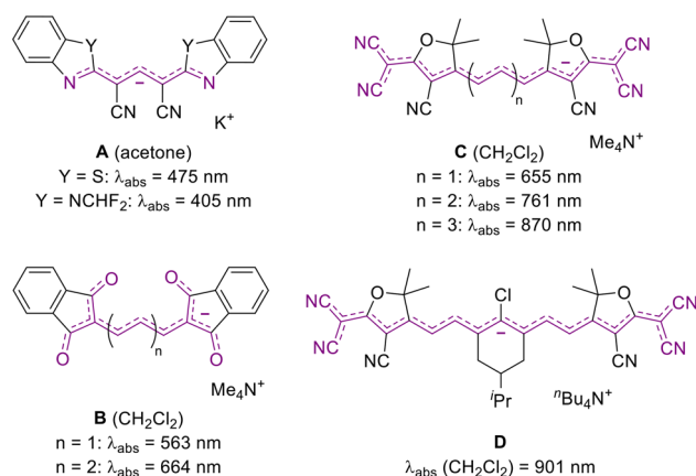
Fig. 1 Optical properties of previously reported anionic polymethines featuring the different end groups.
