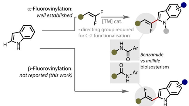
[C] Our strategy: \beta -Fluorovinylation from alkynes via FVI salts
