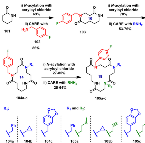
Scheme 9 Iterative N -acylation and CARE reactions.
