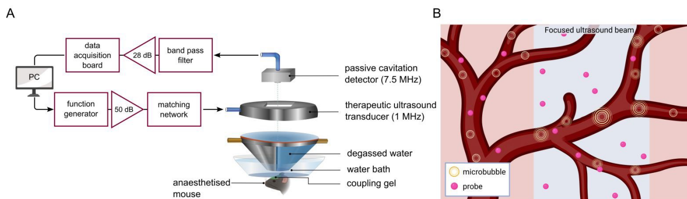
Figure 1. A) In vivo experimental set-up for the focused ultrasound-assisted delivery of Ln.L 2 to the mouse brain. B) Radially-oscillating microbubbles in response to ultrasound exert mechanical stress on the cerebral vasculature to disrupt the blood-brain barrier and enable the crossing of probes into the brain parenchyma. Created in Inkscape and https://BioRender.com .
