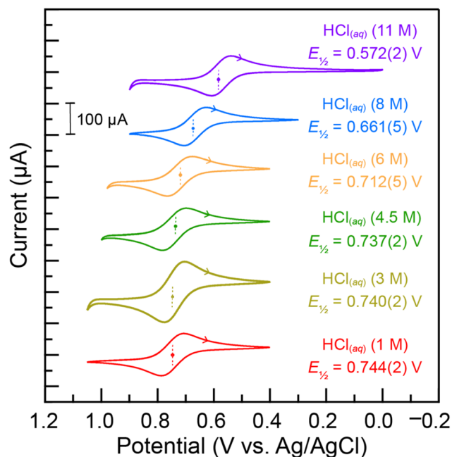
Fig. 5 Cyclic voltammograms from \text{Pu}(\text{IV}) (16.7 mM) dissolved in \text{HCl}_{(\text{aq})} (1–11 M) at a scan rate of 0.01 \text{ V s}^{-1} for the \text{Pu}^{4+/3+}_{(\text{aq})} redox reaction. Data from \text{HCl}_{(\text{aq})} solutions at 1 to 11 M are represented by red, brown, green, orange, blue, and purple traces, respectively. The arrows represent the direction of the potential sweep. The dot with the dashed line indicates the half-wave potential ( E_{1/2} ), which are also provided and referenced to Ag/AgCl. Errors are the standard deviation from three replicates.
