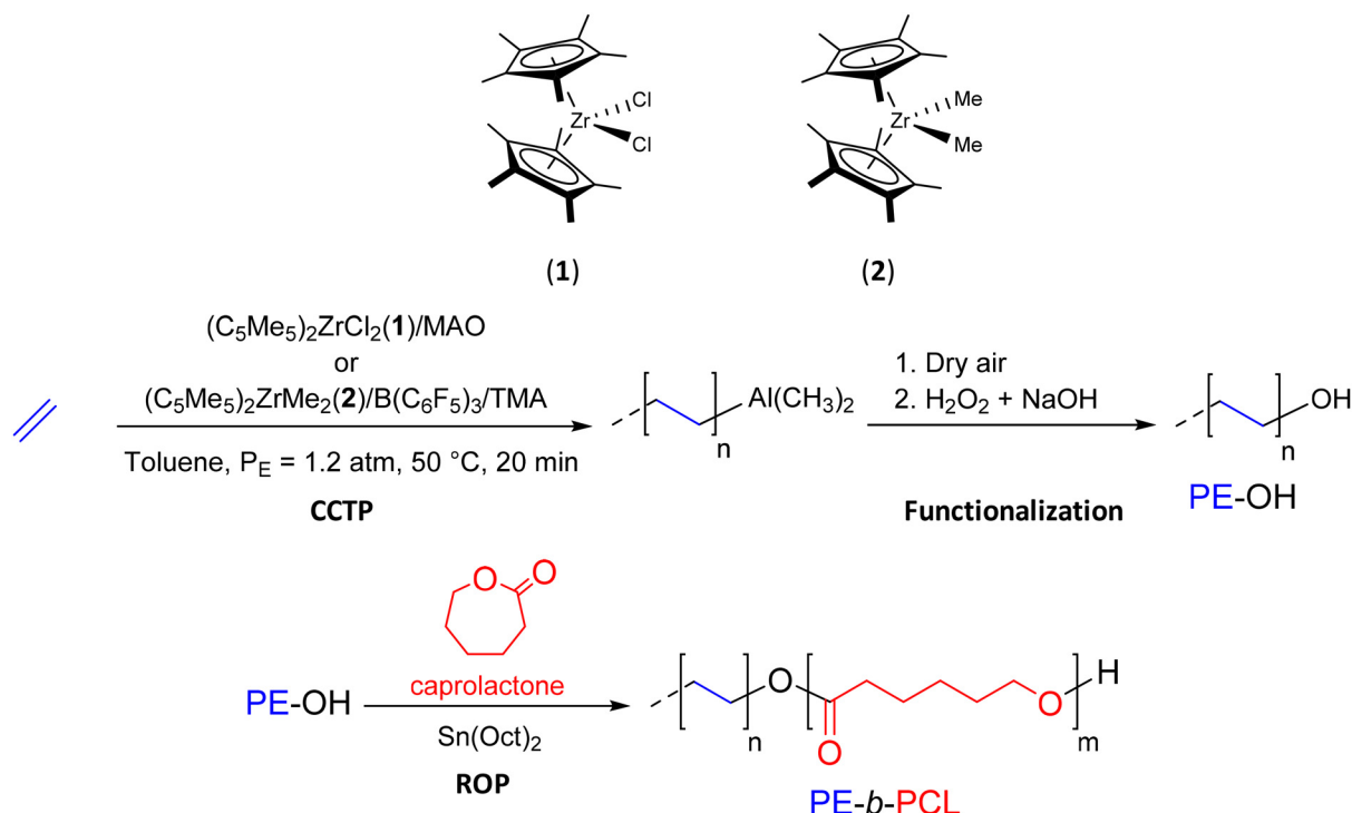
Scheme 3 Synthesis of PE-OH and PE- b -PCL diblock copolymers by successive combination of CTPP and ROP. 24
