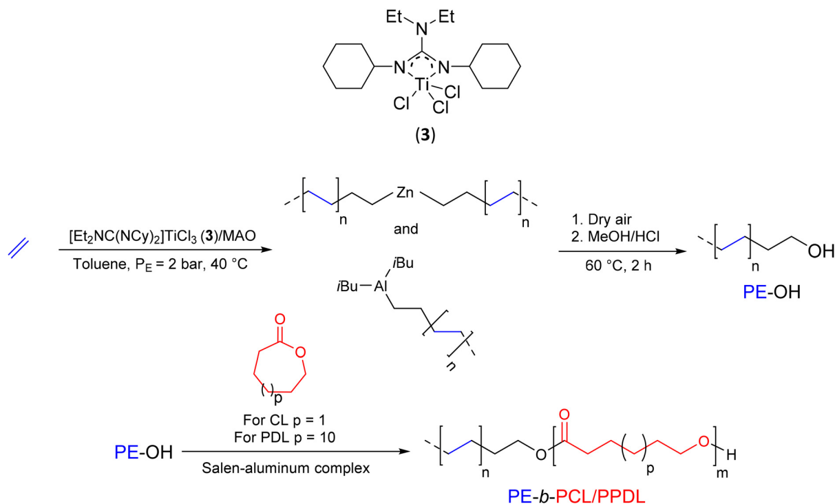
Scheme 4 Synthesis of PE-OH and PE- b -PCL/PPDL diblock copolymers by the combination of CTPP and ROP. 2
