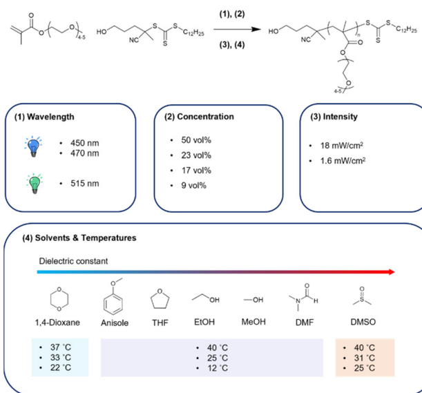
Fig. 1 P(PEGMA) synthesis scheme through the PI-RAFT approach and overview of this study. The synthesis in 1,4-dioxane and DMSO cannot be conducted at 12 °C because of the high melting point of solvents.
