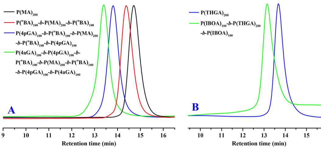
Fig. 5 (A) GPC curves of the PMA homopolymer ( M_n = 19.5 \text{ kg mol}^{-1} , D = 1.02 ), the P^{PIBA} - b -PMA- b - P^{PIBA} triblock ( M_n = 40.5 \text{ kg mol}^{-1} , D = 1.03 ), the P4pGA- b - P^{PIBA} - b -PMA- b - P^{PIBA} - b -P4pGA pentablock ( M_n = 102.3 \text{ kg mol}^{-1} , D = 1.05 ), and P4aGA- b -P4pGA- b - P^{PIBA} - b -PMA- b - P^{PIBA} - b -P4pGA- b -P4aGA ( M_n = 158.5 \text{ kg mol}^{-1} , D = 1.07 ) heptablock copolymers; (B) GPC curves of the PTHGA homopolymer ( M_n = 43.4 \text{ kg mol}^{-1} , D = 1.08 ) and the PIBOA- b -PTHGA- b -PIBOA triblock copolymer ( M_n = 78.4 \text{ kg mol}^{-1} , D = 1.18 ).
