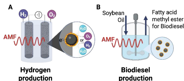
Fig. 10 Use of MH in green fuel production. (A) In hydrogen production, AMFs can activate magnetic catalysts, enhancing water electrolysis by locally increasing reaction temperature and improving electron transfer. (B) In biodiesel production, AMF-induced heating of magnetic nanoparticles accelerates transesterification of oils (e.g., soybean oil) into fatty acid methyl esters, optimizing yield and energy efficiency. Figure created in Biorender.
