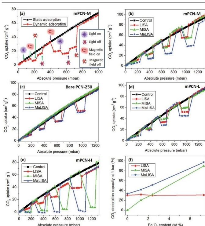
Fig. 11 Successive typical cycles of \text{CO}_2 uptake and release using Metal-organic frameworks (MOFs) called PCN-250 (an Iron-based Porous Coordination Network) with embedded magnetic nanoparticles. The magnetic PCN-250 (mPCN) was used with an increasing content of MNPs ( L < M < H ) ranging from 1.3 wt% (mPCN-L), 2.4 wt% (mPCN-M), to 7.3 wt% (mPCN-H). Three excitation approaches were used: LISA (light-induced swing adsorption), MISA (magnetic induction swing adsorption) and MaLISA (a combination of LISA and MISA) processes. (a) Two successive typical switching cycles of \text{CO}_2 uptake and release in mPCN-M through LISA, MISA and MaLISA processes. (b, c and d and e) dynamic switching of \text{CO}_2 capture and release in mPCN-M (b), bare PCN-250 (c), mPCN-L (d), and mPCN-H (e) by LISA, MISA and MaLISA processes. (f) \text{CO}_2 desorption capacities of mPCNs at 1 bar adapted from the data shown in (b)–(e). All the dynamic \text{CO}_2 adsorption profiles were obtained by intermittently exposing the samples to 365 nm UV light (LISA process) and/or an alternating magnetic field of 17.6 mT and 279 kHz (MISA process) during the \text{CO}_2 adsorption measurement at 298 K. Reproduced from Ref. 162 with permission from the Royal Society of Chemistry.
