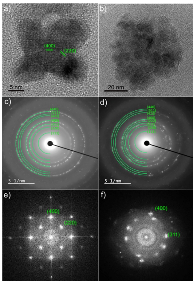
Fig. 2 High-resolution TEM images of (a) 25 nm octopod-shaped Mn-Fe oxide NPs and (b) 50 nm Fe core-Mn shell NPs and their corresponding (c–d) SAED and (e–f) FFT analyses.
