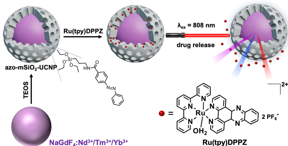
Fig. 1 Preparation of Ru(tpy)DPPZ loaded azo-mSiO 2 -UCNP nanohybrids and NIR-photoactivated drug release. TEOS = tetraethyl orthosilicate; tpy = 2,2':6',2''-terpyridine; DPPZ = dipyrrolo[3,2-a:2',3'-c] phenazine.
