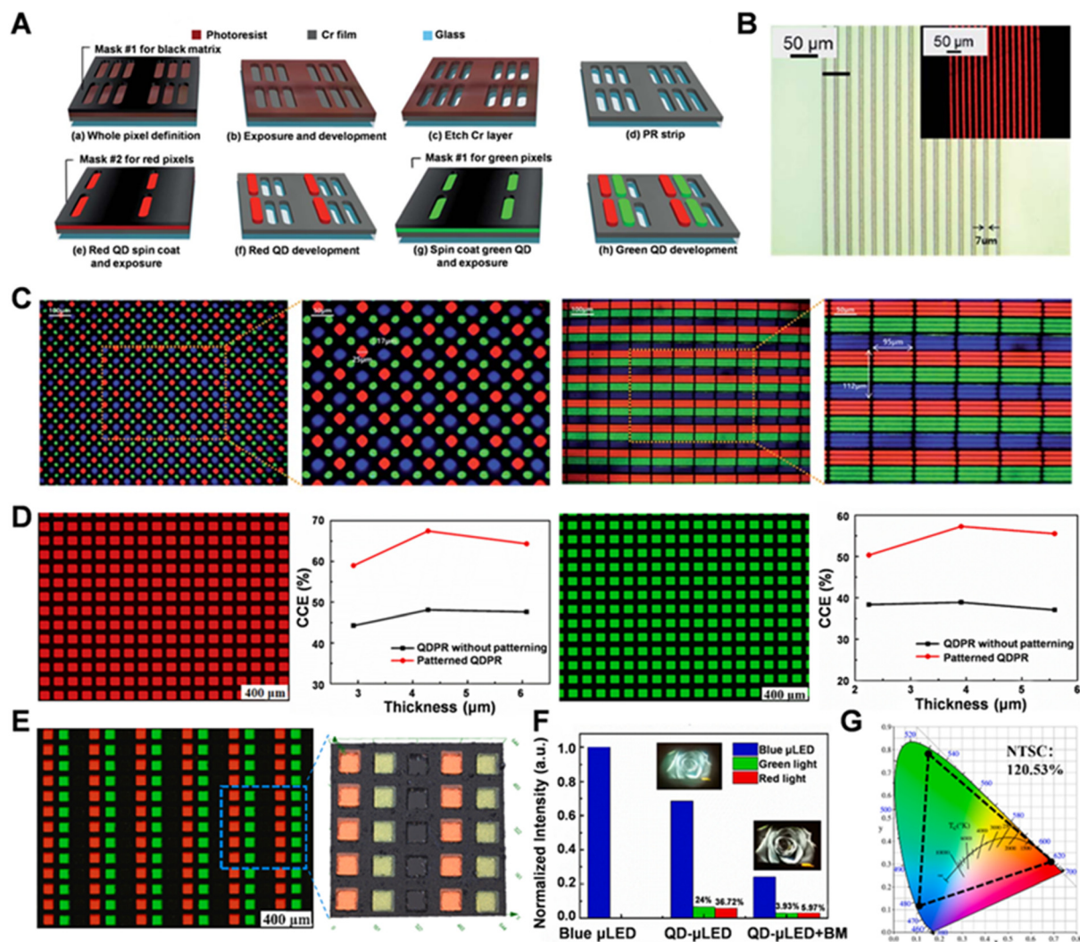
Fig. 9 (A) Schematic of the photolithographic patterning of the QDPR. (B) Microscopy images of the QD patterns with linewidths of 7 μm. (C) Fluorescence images of the RGB QD patterns. Reprinted with permission from ref. 32. Copyright 2022, Royal Society of Chemistry. (D) Fluorescence microscopic images and the CCE of QDPR films with different thicknesses before and after photolithographic patterning. (E) Microscopy images of the red and green two-color QD color conversion arrays. (F) Intensity of blue Micro-LED and color-converted Micro-LEDs with and without a black matrix. (G) Color gamut of the full-color Micro-LED display devices prepared from two-color QD color conversion layers with blue-light Micro-LED. Reprinted with permission from ref. 97. Copyright 2023, Elsevier.
