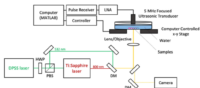
Fig. 4 Schematic illustration of the photoacoustic microscope (PAM) working at 532 and 800 nm. HWP: half-wave plate, PBS: polarizing beam splitter, DM: dichro mirror, LNA: low-noise amplifier.
