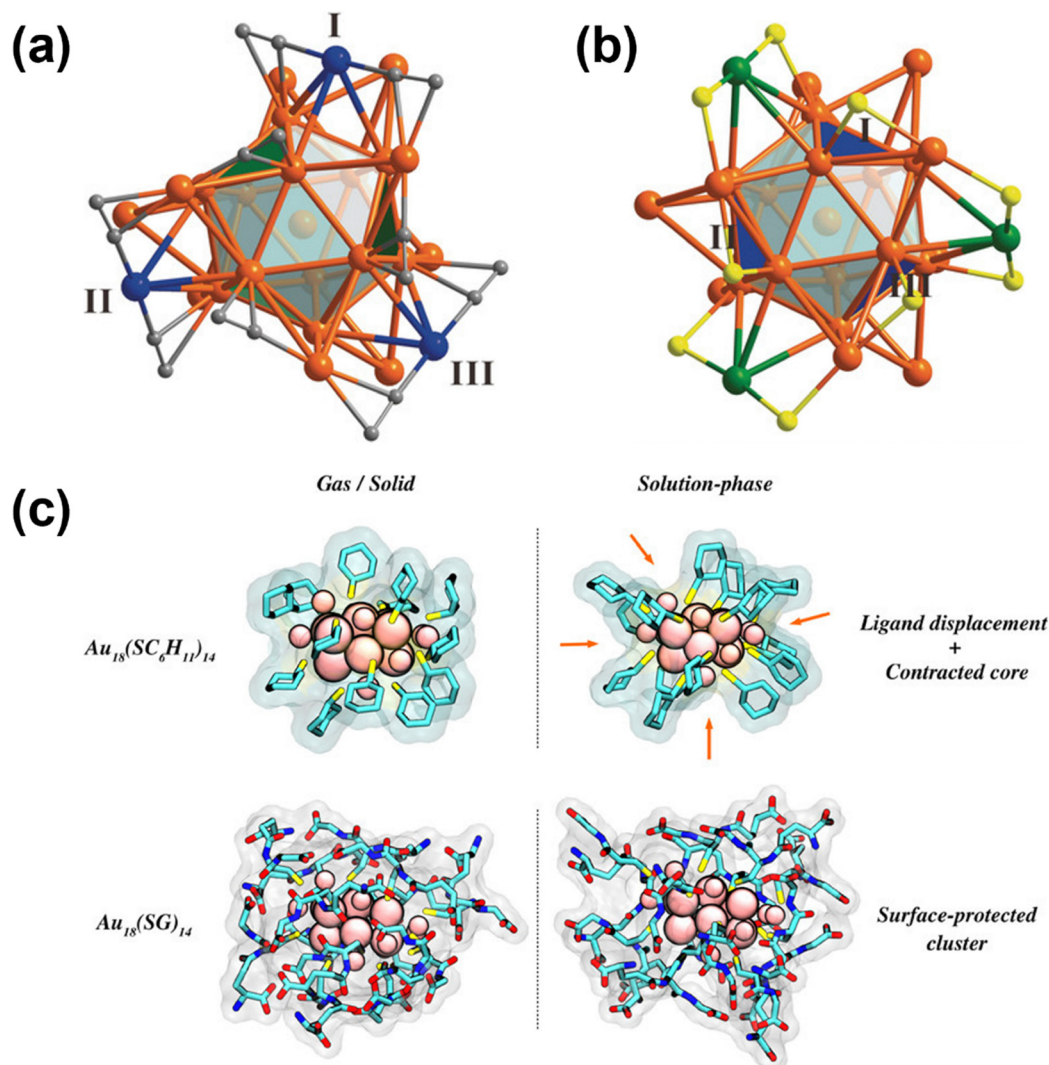
Fig. 5 Illustration of the different arrangements of three V-shaped surface motif staples in (a) alkynyl-protected and (b) thiolate-protected Au_{25} nanoclusters. Colour label: orange, blue and green spheres, Au; yellow spheres, sulfur; grey spheres, carbon. (c). Reprinted with permission from ref. 108. Copyright 2018, Wiley-VCH. Simulated structures of S- c - C_6H_{11} -protected and SG-protected Au_{18}(SR)_{14} in the gas or solution phase. Reprinted with permission from ref. 100. Copyright 2018, American Chemical Society.
