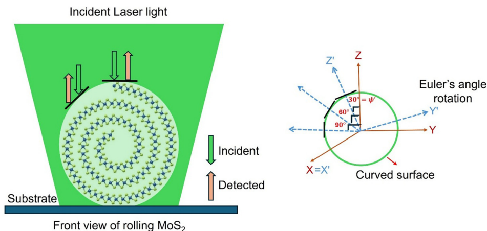
Fig. 6 Illustration of the laser interaction with a rolled surface. Schematic representation of the interaction between a horizontally polarized laser beam and a rolling surface of \text{MoS}_2 , illustrating how changes in the Euler angle ( \psi' ) occur as the beam interacts with different curved regions of the rolling surface. This setup demonstrates the variation in light incidence across the rolling surface.
