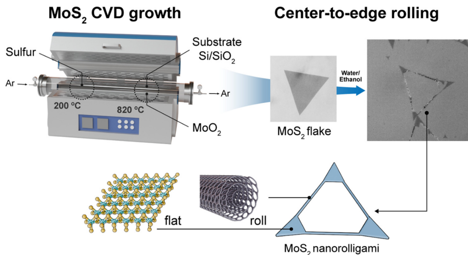
Fig. 1 Step-by-step description of the nanorolligami process. In the first step, the monolayer (1-L) \text{MoS}_2 is prepared via the CVD technique. The second step is to roll the 1-L \text{MoS}_2 by dripping a solution of water and ethanol in a 2 : 1 ratio at room temperature (RT). The solution causes a strong mechanical strain in the central part of the 1-L \text{MoS}_2 , resulting in a break from the center and self-rolling at each corner. The in situ video of self-rolling \text{MoS}_2 has been recorded using a microscope.
