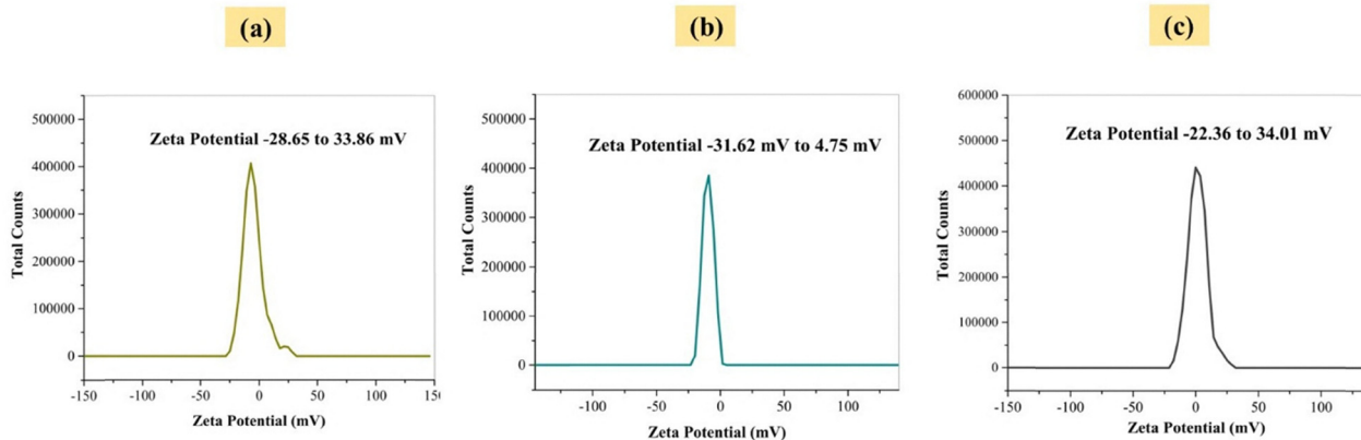
Fig. 6 Zeta potential distribution curves for (a) sample A, (b) sample B, and (c) sample C.
