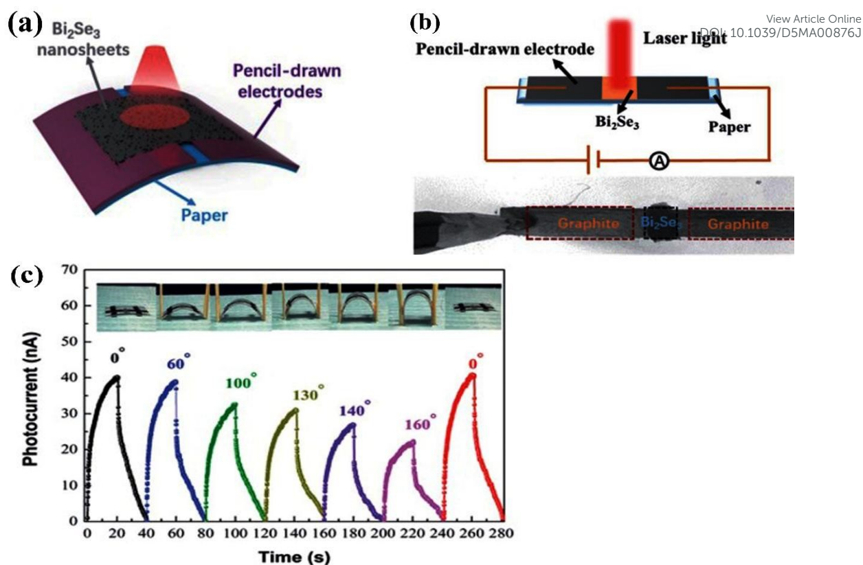
Fig. 13 a) Schematic of the bismuth selenide infrared photodetector device based on the flexible paper substrate, b) illustration of the corresponding photocurrent measurement, c) photocurrent rise and decay time (response time) under consecutive turning on/off of the incident light under different bending conditions. reprinted with permission from ref 124 .
