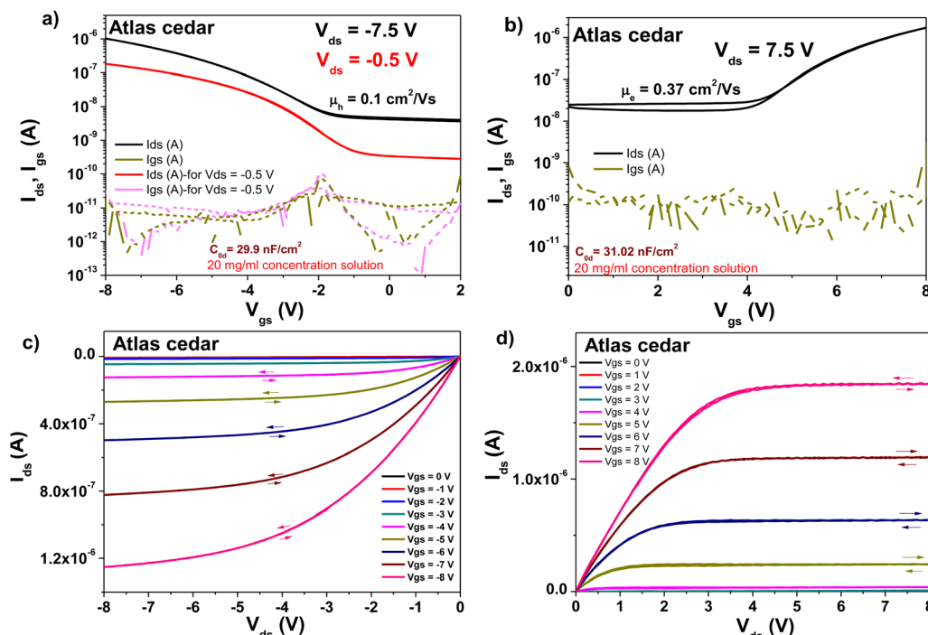
Fig. 15 Transistor measurements of Atlas cedar resin on 10 V anodized aluminum gate electrode (i.e., \sim 16 – 17 nm thick aluminum oxide, Al_2O_3 ) with pentacene and C 60 as the organic semiconductor: (a) transfer curve of the OFET using pentacene as organic semiconductor. (b) Transfer curve of the OFET using C 60 as the organic semiconductor. (c) Output curve of the OFET using pentacene as the organic semiconductor. (d) Output curve using C 60 as the organic semiconductor.
