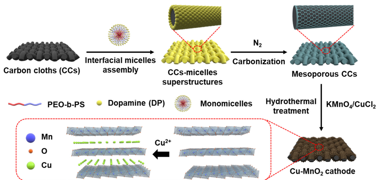
Fig. 1 Synthesis of \text{Cu-MnO}_2 (schematic).
