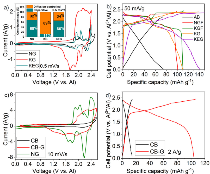
Fig. 7 (a) CV curves of cells with natural graphite (NG), 59 Kish graphite (KG) 61 and kish-based expanded graphite (KEG) 17 cathode and \text{AlCl}_3/[\text{EMIM}]\text{Cl} (1.3:1) electrolyte, at a scan rate of 0.5 \text{mV s}^{-1} . Insert is the contribution ratio of these three graphite cathodes. (b) Charging and discharging profiles of cells with various graphitic materials and \text{AlCl}_3/[\text{EMIM}]\text{Cl} (1.3:1) electrolyte at 50 \text{mA g}^{-1} . These graphite materials are KG 61 and KEG, 17 and kish graphite flakes (KGF, 2 mm), natural large graphite flakes (NGF, 1 mm) and acetylene black (AB, 26 \mu\text{m} ). 19 (c) CV curves at a scan rate of 10 \text{mV s}^{-1} and (d) charging/discharging profiles at a current density of 2 \text{A g}^{-1} of cells with NG 59 (only used in CV), CB (XC-72) and CB-G (carbon black-derived nanosheet-bricked porous graphite, NSPG-120) 66 cathode and \text{AlCl}_3/[\text{EMIM}]\text{Cl} (1.3:1) electrolyte. Adapted with permission from Elsevier. 17 Copyright 2024. Adapted with permission from author. 19 Copyright 2017. Adapted with permission from Springer Nature. 59 Copyright 2024. Adapted with permission from Elsevier. 61 Copyright 2023. Adapted with permission from author. 66 Copyright 2018.
