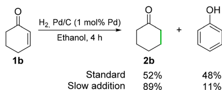
Fig. 3 Hydrogenation of 2-cyclohexenone ( 1b ) with Pd/C and \text{H}_2 .
