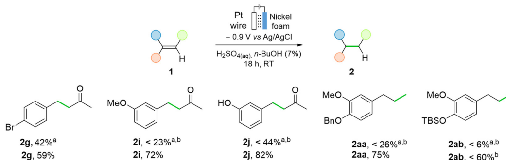
Fig. 10 Substrate scope and limitations using n\text{BuOH} as cosolvent instead of EtOH. 1 (0.4 mmol, 0.016 M). a Using aqueous \text{H}_2\text{SO}_4 (0.19 M)/EtOH (3 : 1). b Yields were determined by ^1\text{H} NMR spectroscopy using an internal standard.
