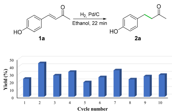
Fig. 4 Recyclability performance of the Pd/C and \text{H}_2 method at low conversions, after reaction times of 22 min. Yields were determined by ^1\text{H} NMR spectroscopy using an internal standard.
