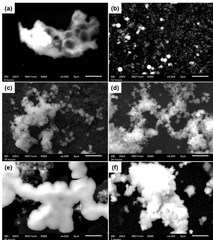
Fig. 9 Typical scanning electron microscopy (SEM) images of the SiN windows with deposited P 11 -4 that were imaged on the I14 beamline (magnification = ×4000). (a) 6 hours, (b) 12 hours, (c) 16 hours, (d) 24 hours, (e) 48 hours and (f) 2 weeks. The secondary electron detector was used at an energy of 20 kV, a working distance of 11 mm and a spot size of 60 nm.
