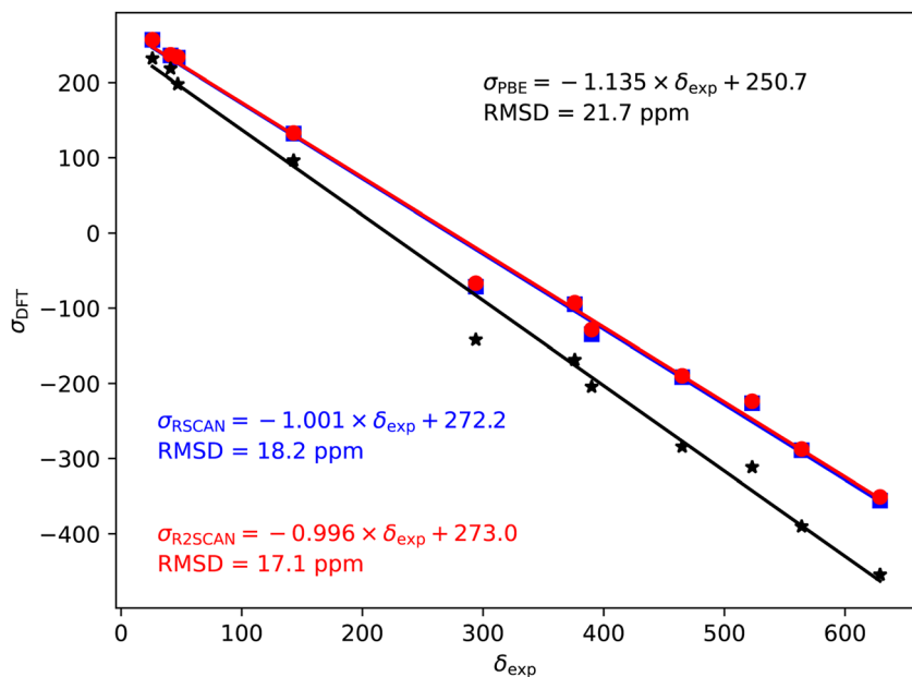
Fig. 3 ^{17}\text{O} magnetic shieldings, \sigma , calculated with the PBE (black), rSCAN (blue) and r^2\text{SCAN} (red) functionals vs. experimental chemical shifts, \delta . For each functional the line of best fit is given.
