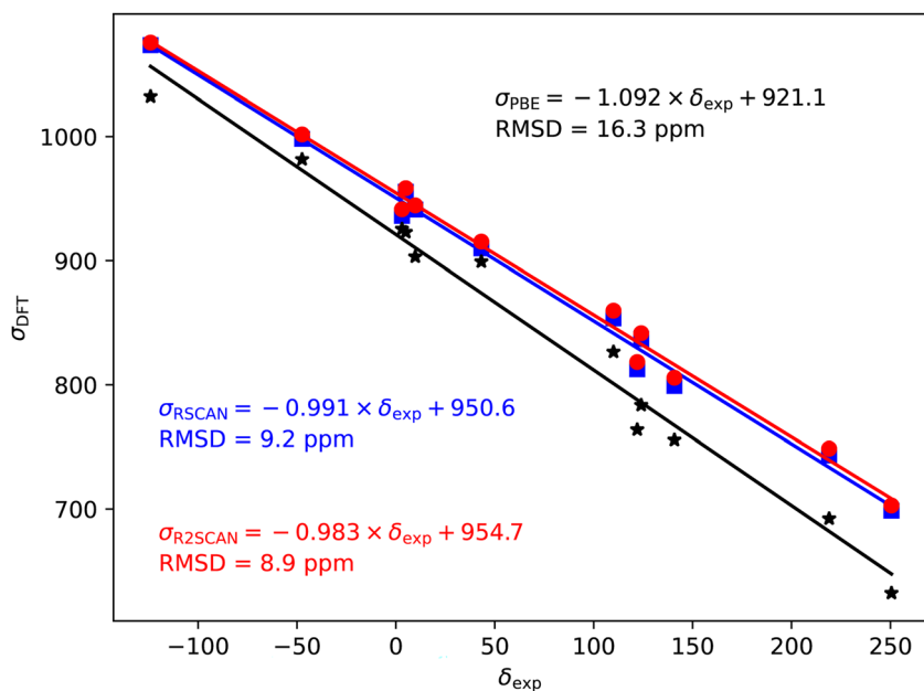
Fig. 4 ^{35/37}\text{Cl} magnetic shieldings, \sigma , calculated with the PBE (black), rSCAN (blue) and r^2\text{SCAN} (red) functionals vs. experimental chemical shifts, \delta . For each functional the line of best fit is given.
