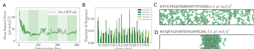
Fig. 5 Optimisation using Expected Improvement (EI) acquisition function to find the optimal value of -B_{22} . (A) Evolution of mean squared error (MSE) between the predicted and expected -B_{22} of the ProteinGPT2 validation set. (B) Fraction of amino acids in the sequences suggested by Wazy after each iteration. (C) Snapshot of the simulations of sequences suggested by wazy at the 4th iteration. (D) The sequences with more negative B_{22} showed clear phase separation (Fig. S2B†).
