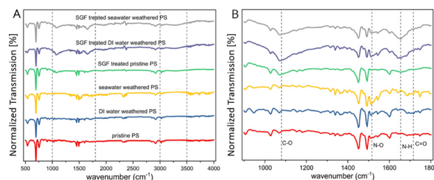
Fig. 1 ATR-FTIR spectrum of surface chemical functional groups on all particles. A. Spectrum of all types of particles at full wavenumber range from 500–4000 \text{cm}^{-1} and B. spectrum of wavenumber range from 900–1800 \text{cm}^{-1} .
