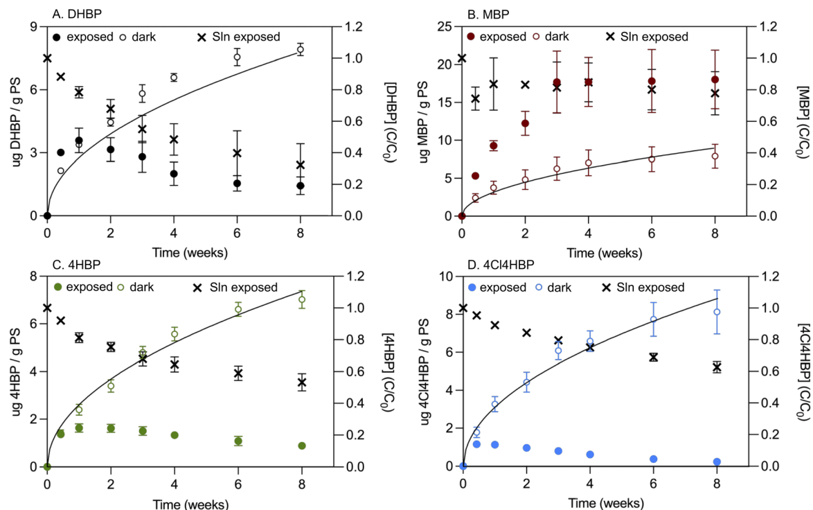
Fig. 2 Concentration of (A) DHPBP, (B) MBP, (C) 4HBP, and (D) 4Cl4HBP detected in the leachate solutions of 1 w/w% benzophenone-PS composites ( n = 3 ) suspended in water and exposed to sunlight (closed circles) for 8 weeks or kept under dark conditions (open circles). Overlaid is the photodegradation kinetics of the additives in solution ( 10 \text{ mg L}^{-1} ) exposed to the same sunlight conditions (labeled as Sln exposed and indicated with black crosses) and collected at the same times as the aliquots from the benzophenone-PS composites. The solid lines in each plot represent the best fit data for the passive release of benzophenones from PS using a kinetic model where the rate of release is proportional to release time ( t^{0.5} ). Note the different y-axis scale for MBP as compared to the other three BP additives. It should be noted that the exposure time represents the time span of sunlight exposure.
