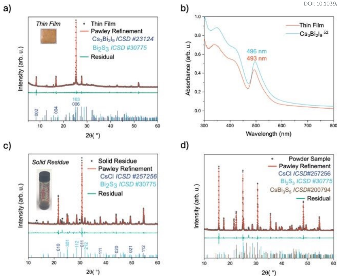
Figure 3. Challenges with CsBiSbCl 2 synthesis (a) PXRD pattern of thin films synthesized according to Huang et al. (solid circles), with the corresponding Pawley refinement to Cs 3 Bi 2 I 9 and Bi 2 S 3 (red line); Rwp = 9.1874 GoF = 1.2124. Inset: Photograph of the as-prepared thin film on 1.4 cm 2 glass. (b) UV-Vis absorption spectrum of prepared thin films and Cs 3 Bi 2 I 9 reference spectrum, 52 with the characteristic Cs 3 Bi 2 I 9 excitonic peaks labelled. (c) PXRD pattern of solid residue from precursor solution from the attempted synthesis of CsBiSbCl 2 (solid circles), with the corresponding Pawley refinement to Bi 2 S 3 and CsCl (red line); Rwp = 12.9970 GoF = 2.1417, unidentified peaks are labelled by *. Inset: Photograph of the solid residue in a glass vial. (d) PXRD pattern of material from attempted solid-state synthesis of CsBiSbCl 2 (solid circles), with the corresponding Pawley refinement to CsCl, Bi 2 S 3 , and CsBi 3 S 5 (red line); Rwp = 10.9693, GoF = 1.7417.
