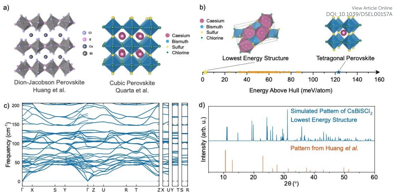
Figure 1. Structure of CsBiS 2 (a) Proposed crystal structure of CsBiS 2 by Huang et al. 17 and Quarta et al. 33 Illustration of structure proposed Huang et al. reprinted with permission from J. Huang et al. , J. Phys. Chem. Lett. , 2024, 15 , 3383–3389. Cubic perovskite structure prepared from the information provided in Ref. 33. (b) Energy above the Cs-Bi-S-Cl convex hull of CsBiS 2 structures selected for DFT refinalization. Shown are the lowest energy structure (yellow star), tetragonal perovskite structure (blue star), and remaining CsBiS 2 structures within 70 meV/atom of the hull (orange circles). (c) Phonon dispersion curve of the lowest-energy CsBiS 2 structure found from AirSS. Lack of imaginary modes ( i.e. , no negative frequencies) demonstrates the dynamic stability of this structure. (d) Comparison of the simulated powder X-ray diffraction (PXRD) pattern for the lowest energy Pnma structure and the CsBiS 2 PXRD pattern reported by Huang et al. 17 Comparison with tetragonal perovskite reference pattern shown in Fig. S6, SI.
