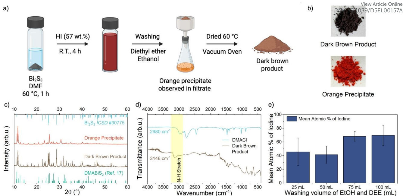
Figure 2. Preparation of DMABiS 2 Intermediate. (a) Illustration of the synthesis procedure for preparation of the DMABiS 2 intermediate. Created in BioRender. Quinn, E. (2025) https://BioRender.com/xo6o9y9 (b) Images of the dark brown product powder and the orange precipitate observed in the filtrate during the washing stage. (c) PXRD pattern of synthesized DMABiS 2 material. The light blue bars indicate the reference patterns of Bi 2 S 3 (ICSD #30775), while the light green bars represent the reported pattern by Huang et al. for their claimed DMABiS 2 intermediate. (d) Infrared spectra of the dark brown powder and DMABiS 2 reference material. The peaks assigned to the ammonium N-H stretch are highlighted. The increase in peak wavenumber for the dark brown powder sample is attributed to the reduction in electronegativity of the environment leading to stronger N-H bonds. (e) The effect of solvent washing volume on the mean atomic percentage of iodine from EDS measurements of dark brown product powders. The error of atomic percentage is calculated using procedure described in Fig. S12, SI.
