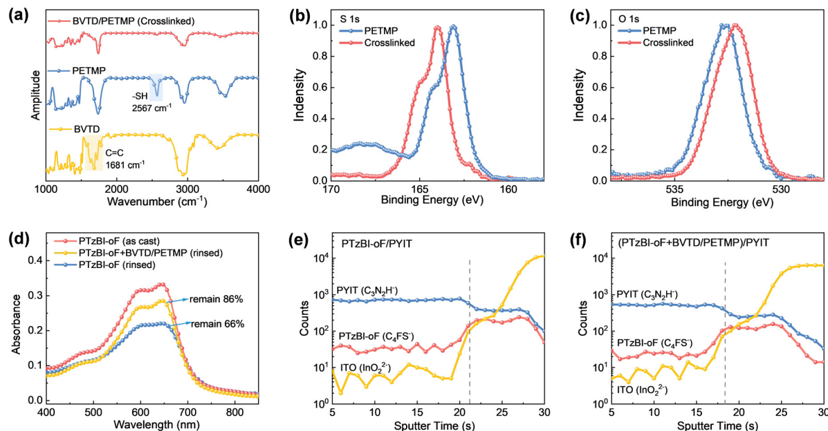
Fig. 2 (a) FTIR spectra of BVTd, PETMP, and their 2:1 (wt:wt) blend film after the thiol-ene click reaction. (b) and (c) XPS spectra of the S 1s and O 1s core levels for PETMP and the crosslinked network. (d) Normalized UV-vis absorption spectra of as-cast PTzBI-oF films and CF-rinsed films, with and without the crosslinked network (prepared using 4 wt% BVTd relative to PTzBI-oF). TOF-SIMS depth profiles of the PTzBI-oF/PYIT active layers, (e) with and (f) without the crosslinked network, where the grey dotted lines indicate the interface between the active layers and the ITO substrate.
