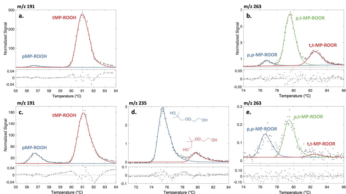
Fig. 1 Representative chromatograms of ROOH (a and c) and ROOR (b, d, and e.) products formed in the oxidation of 2-methylpropene in experiments with high RO 2 /HO 2 ratios (top row) and high HO 2 /RO 2 ratios (bottom row). Experiments represented in the bottom row also included ethene. The experimentally measured signal is given as dark gray dots, while the colored lines are the bootstrap best fits of the chromatographic data. The corresponding structures are the assignments of these peaks. Below each chromatogram are plots of the residuals of the best fits given as fractions of the maximum peak value.
