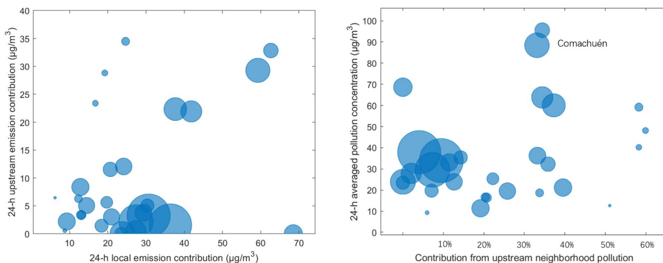
Fig. 10 Baseline scenario (a). Comparison of the local emitted \text{PM}_{2.5} concentration and the upstream neighborhood emitted concentration (b). Contribution from neighborhood pollution in different communities. Note: bubbles are scaled to represent number of homes in each community.
