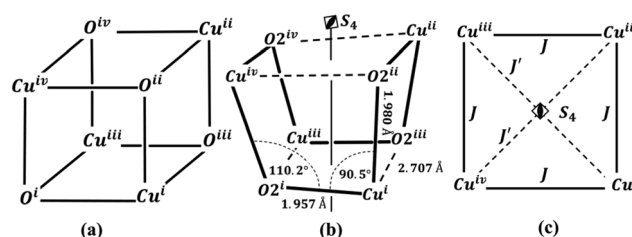
Fig. 6 (a) Ideal cubane Cu 4 O 4 core ( T_d symmetry). (b) Cubane-like Cu 4 O 4 core in the tetranuclear Cu 4 L 4 complex (crystallographic site symmetry S_4 , a subgroup of T_d ) showing super-exchange relevant Cu–O bond paths (in full lines), distances (Å) and Cu–O–Cu bond angles ( ^\circ ). Some weaker Cu...O paths are indicated by thin lines. Symmetry operations as in Fig. 3. (c) Exchange coupling scheme used in the spin Hamiltonian of eqn (2).
