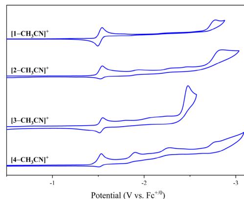
Fig. 2 Cyclic voltammograms of 1 mM [\mathbf{1-CH_3CN}]^+ , [\mathbf{2-CH_3CN}]^+ , [\mathbf{3-CH_3CN}]^+ and [\mathbf{4-CH_3CN}]^+ recorded in argon-saturated 0.1 M [\text{Bu}_4\text{N}][\text{PF}_6] acetonitrile supporting electrolyte at a glassy carbon electrode with a scan rate of 0.1 \text{ V s}^{-1} .
