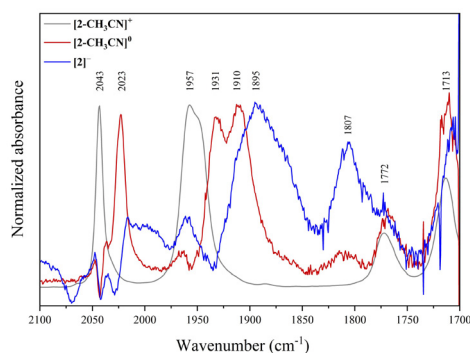
Fig. 3 IRSEC results upon controlled potential electrolysis of [2\text{-CH}_3\text{CN}]^+ recorded in argon-saturated 0.1 \text{ M} [\text{Bu}_4\text{N}][\text{PF}_6] acetonitrile supporting electrolyte.
