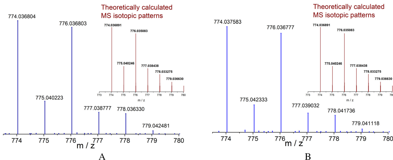
Fig. 3 HRMS-ESI spectra obtained by the positive scan of 1 (A) and 2 (B) in \text{CH}_3\text{OH} –water (1:1, v/v). Insets: calculated isotopic distribution for monocationic dinuclear complexes: [\text{Cu}_2(4,4'\text{-dmbp})_2(\text{HRis})]^+ and [\text{Cu}_2(5,5'\text{-dmbp})_2(\text{HRis})]^+ .
