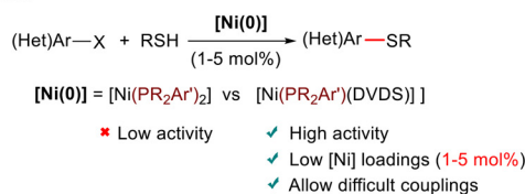
Scheme 1 (A) Our previous work on C–S cross-coupling using pre-formed \text{Ni}(\text{II}) -allyl precatalysts with terphenyl phosphine ligands. (B) \text{P}_2\text{Ni}(0) complexes with monophosphine ligands. (c) This work.
