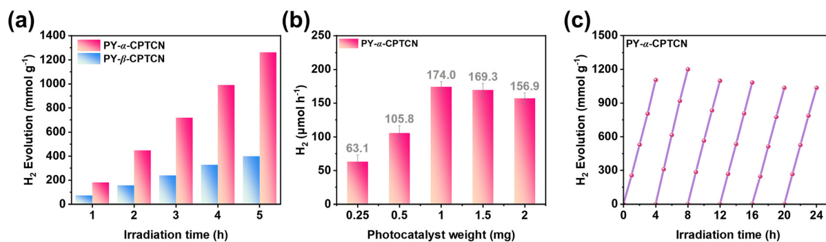
Fig. 2 (a) Hydrogen evolution versus time of PY- \alpha -CPTCN and PY- \beta -CPTCN NPs at the concentration of 5 \text{ }\mu\text{g mL}^{-1} , under AM 1.5G ( 100 \text{ mW cm}^{-2} ). (b) Photocatalytic \text{H}_2 evolution patterns of PY- \alpha -CPTCN NPs with different weights of the photocatalyst. (c) Time course hydrogen evolution curve of PY- \alpha -CPTCN NPs.
