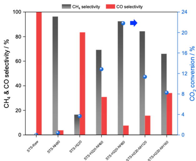
Fig. 1 CO 2 methanation performance of STS powder samples before and after each treatment step. Reaction conditions: T = 300\text{ }^{\circ}\text{C} , P = 1\text{ bar} , flow rate = 20 mL min -1 , reaction gas = H 2 /CO 2 /N 2 = 64/16/20.
