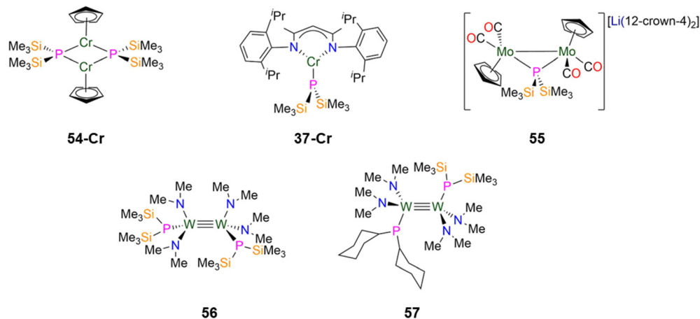
Fig. 15 Group 6 P'' complexes [Cr(Cp)(\mu-P'')]_2 ( 54-Cr ), [Cr(D^{iPr}P''Nacnac)(P'')] ( 37-Cr ; D^{iPr}P''Nacnac = CH((CH_3)_2CN(Dipp))_2 ; Dipp = C_6H_3^iPr_2-2,6 ), [Li(12-crown-4)]\{[Mo(Cp)(CO)_2]_2(\mu-P'')\} ( 55 ), [1,2-W_2(P'')(NMe_2)_4] ( 56 ), [1,2-W_2(PCy_2)(P'')(NMe_2)_4] ( 57 ).
