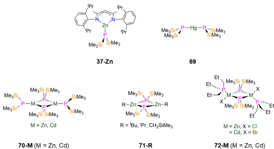
Fig. 20 Monomeric and dimeric group 12 P'' complexes [\text{Zn}(\text{DippNacnac})(P'')] ( 37-Zn ; \text{DippNacnac} = \text{CH}((\text{CH}_3)_2\text{CN}(\text{Dipp}))_2 ; \text{Dipp} = \text{C}_6\text{H}_3\text{iPr}_2\text{-2,6} ), [\text{Hg}(P'')]_2 ( 69 ), [\text{M}(P'')(\mu\text{-}P'')]_2 ( 70-M , M = Zn, Cd ), [\text{Zn}(\text{R})(\mu\text{-}P'')]_2 ( 71-R , \text{R} = \text{tBu}, \text{iPr}, \text{CH}_2\text{SiMe}_3 ), [\text{M}(P''\text{Pr}_3)(\text{X})(\mu\text{-}P'')]_2 ( 72-Zn : M = Zn, X = \text{Cl} ; 72-Cd : M = Cd, X = \text{Br} ).
