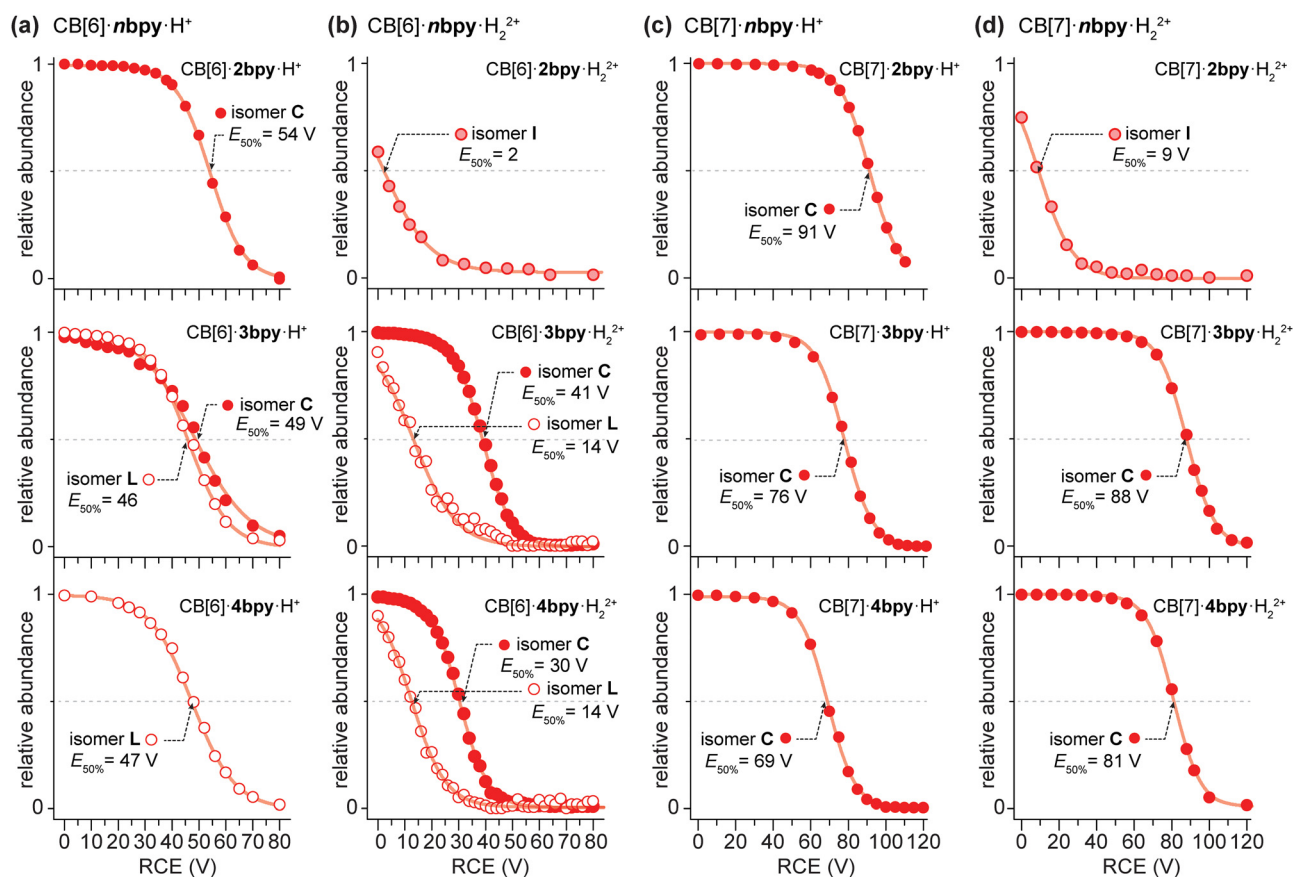
Fig. 3 The energy-dependent survival yield of precursor ions, the singly- and doubly-protonated \text{CB}[x]\cdot\text{bipyridine} complexes ( x = 6 or 7 ): (a) \text{CB}[6]\cdot n\text{bpy}\cdot\text{H}^+ , (b) \text{CB}[6]\cdot n\text{bpy}\cdot\text{H}_2^{2+} , (c) \text{CB}[7]\cdot n\text{bpy}\cdot\text{H}^+ , and (d) \text{CB}[7]\cdot n\text{bpy}\cdot\text{H}_2^{2+} ( n = 2, 3 , and 4 for top, middle, and bottom, respectively). Red lines denote the sigmoidal fits of the precursor ( \text{CB}[x]\cdot\text{bipyridine} complex ions) depletion. RCE denotes the relative collision energy ( \text{RCE} = z \cdot V_{\text{CE}} ), where z is the charge state of complex ion and V_{\text{CE}} is acceleration voltage before entering the collision cell. For each isomer, the RCE for 50% precursor dissociation ( E_{50\%} ) value is shown together.
