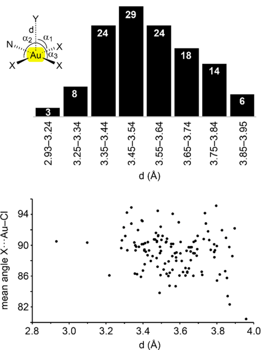
Fig. 13 Top: Histogram showing the distribution of CSD hits as a function of the Y \cdots Au distance. Bottom: Scatterplot of the mean Y \cdots Au–Cl angle ( \alpha ) versus the Y \cdots Au distance.
