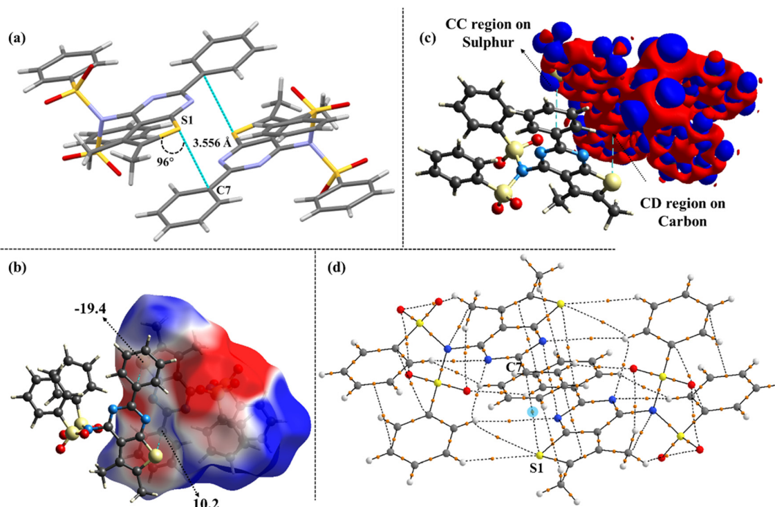
Fig. 16 (a) Distance and directionality of S...C ( \pi -hole) tetrel interactions in compound 11 ; (b) MESP mapped over the Hirshfeld surface (values in \text{kJ mol}^{-1} ); (c) deformation density plot depicting the CC and CD regions; (d) QTAIM analysis validates the existence of bond critical points (highlighted in blue circles) in dimeric motifs.
