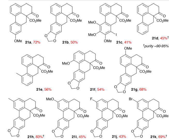
Scheme 4 Photocyclisations of 1-( o -iodobenzyl)-2-tetralones give benzanthracenones in moderate to good yield.
