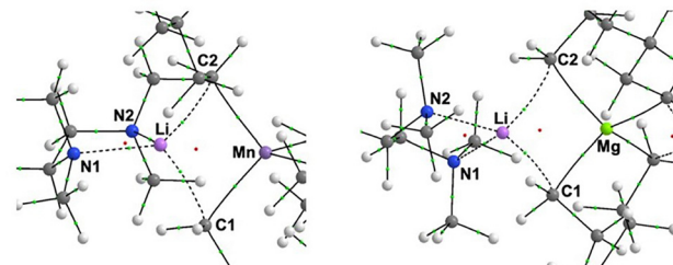
Fig. 2 Molecular graph for 1 (left) and 2 (right). BCPs (green dots) and RCPs (red dots) shown along with bond paths.
