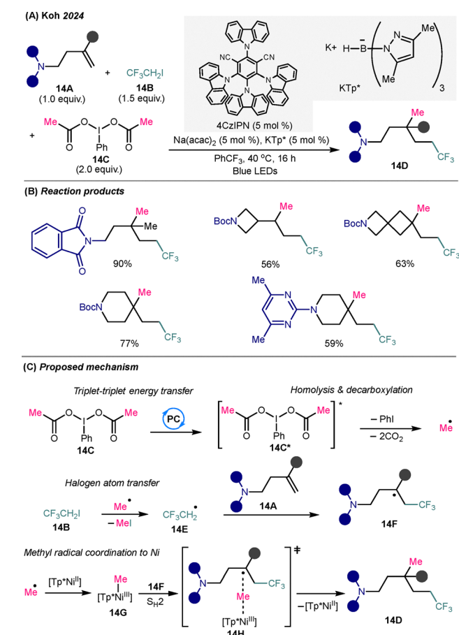
Scheme 14 Dual nickel/photoredox-catalyzed methyl-trifluoroethylation of amino-substituted alkyl alkenes. (A) General reaction conditions. (B) Representative substrate scope. (C) Proposed mechanism.
